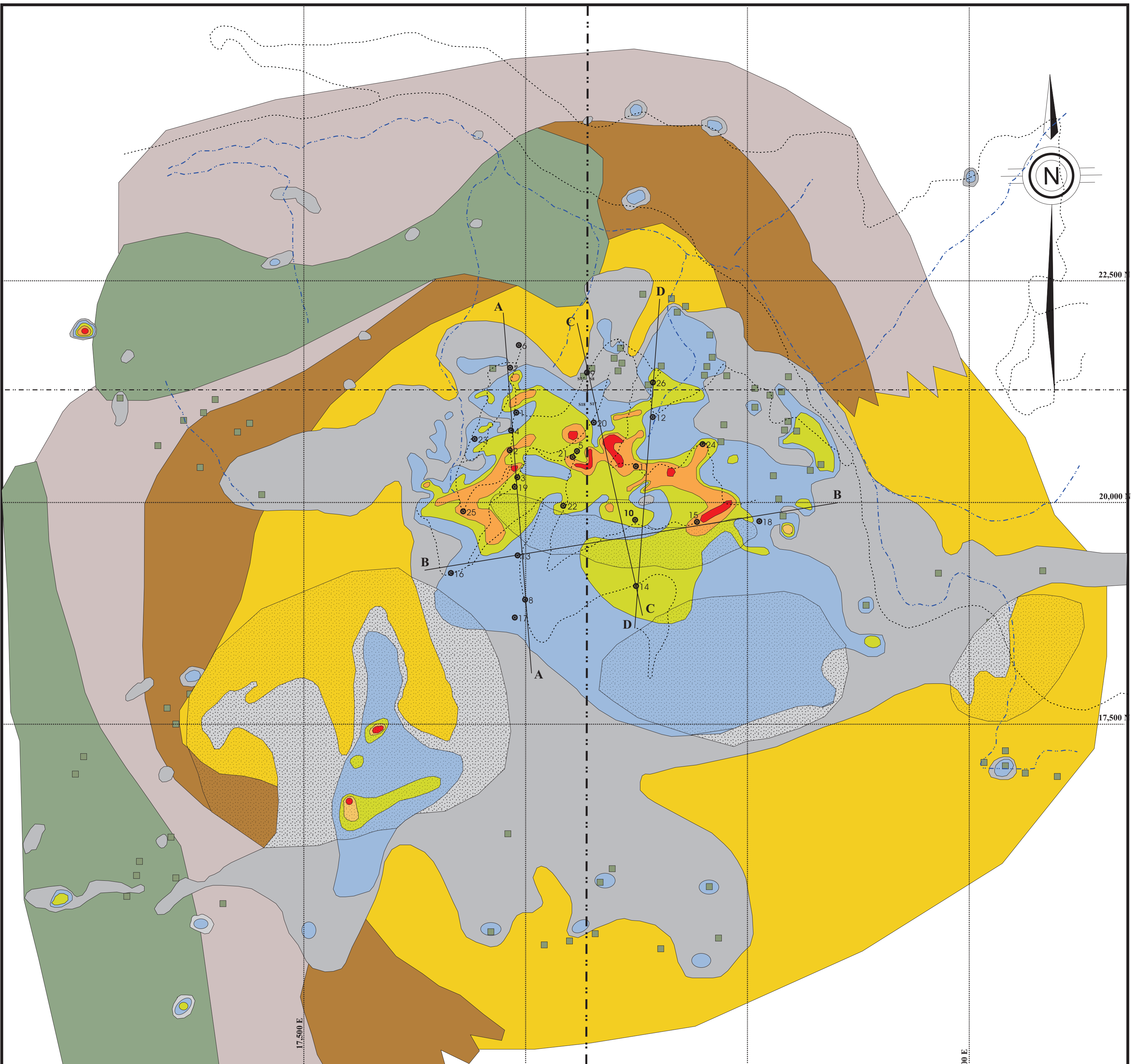
Surface Distribution of Quartz and Epidote Vein Observation; and Metal zonation based on Copper, Lead and Zinc Modified from D. J. Baker, 1983 plates 10,19 and 33
